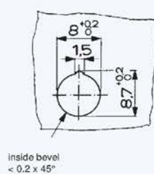
Front panel drilling
