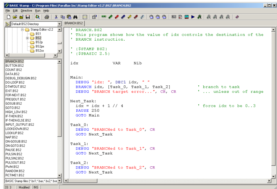
Figure 3.1: BASIC Stamp Windows Editor.
