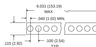
CTA4-.100(2.54) Centers
