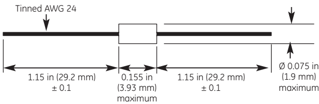
NTC Type GE dimensions
