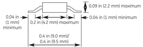
NTC Type DKM wires should not be bent within 0.08 in (2 mm) of glass body
