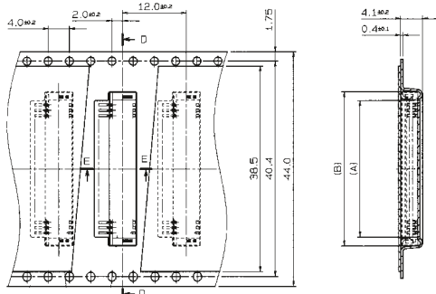
SECT. D-D
