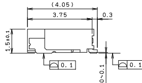
SECT. D-D
