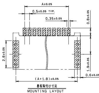
MOUNTING LAYOUT
