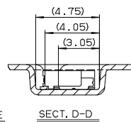
SECT. D-D
