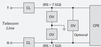
Suggested Arrangement to Meet TIA-968-A for a Grounded CPE Design
