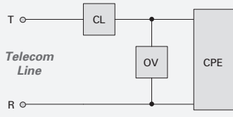
Suggested Arrangement to Meet TIA-968-A for a Ungrounded CPE Design
