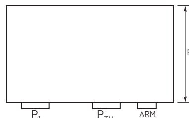
Figure RTP7-RTP8 Dimension Figures for RTP140R060S Devices
