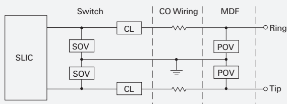
Simplified Model of Central Office End of Subscriber Loop
