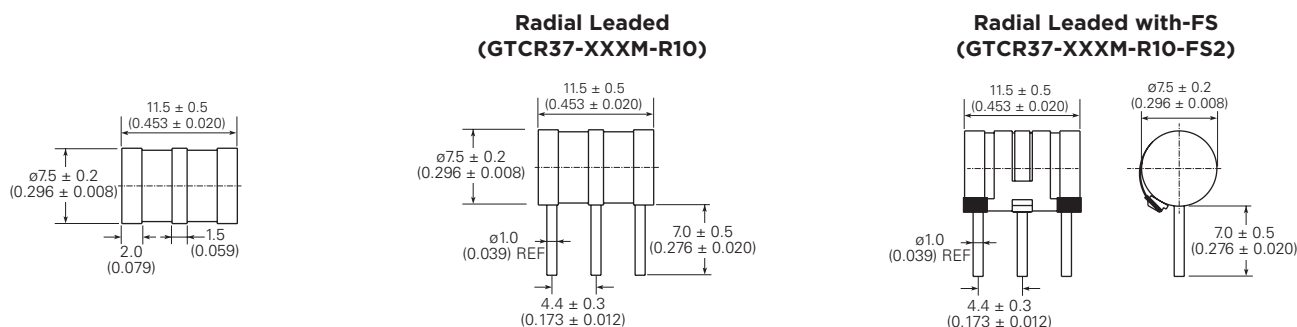
Figure G10 Three Electrode 7mm Product Dimensions
