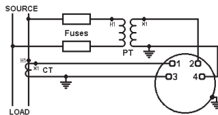
Fig. 21 Models 077-215, 077-KHB 078-215J, 078-KHBJ, 079-215 Wattmeter Single Phase.
