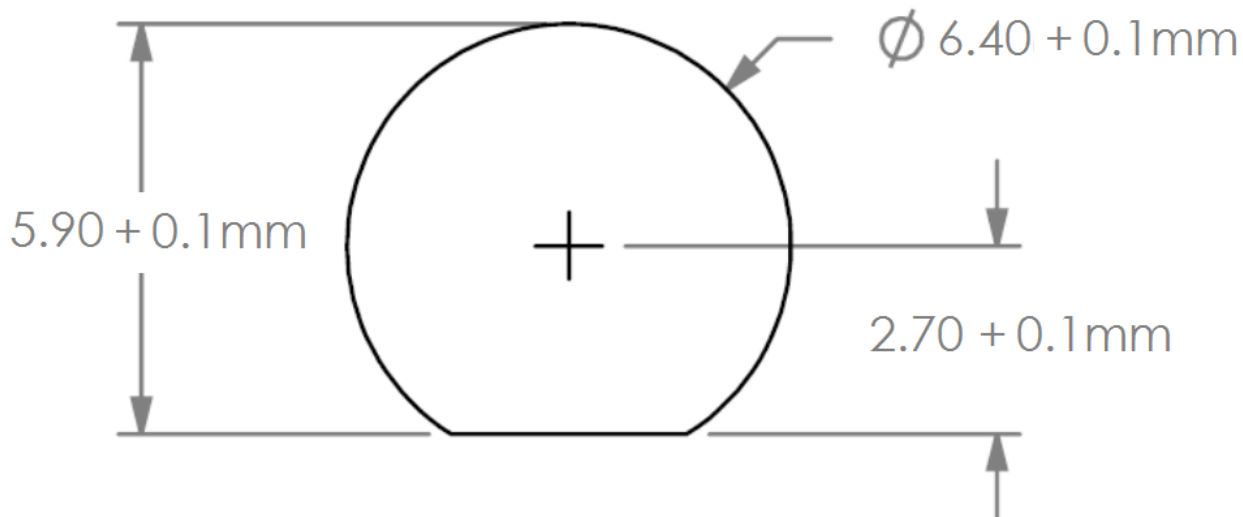
Figure 2 Recommend Cutout
