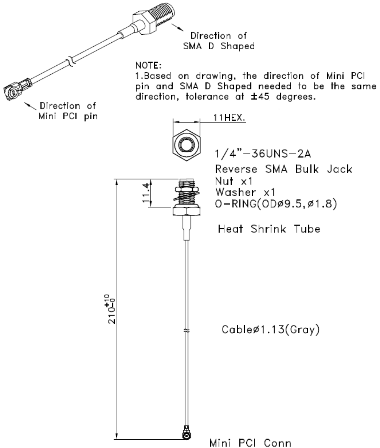
Figure 1 Physical Dimensions
