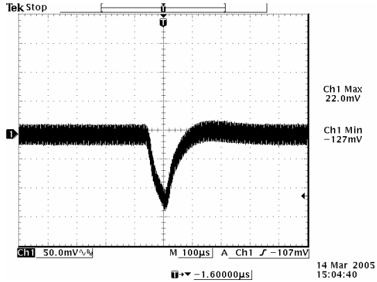
Transients 25% to 50% load 1.8 Vdc output
