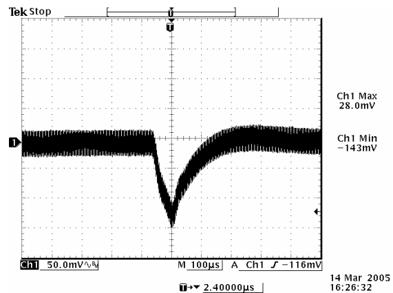
Transients 25% to 50% load 2.5 Vdc output
