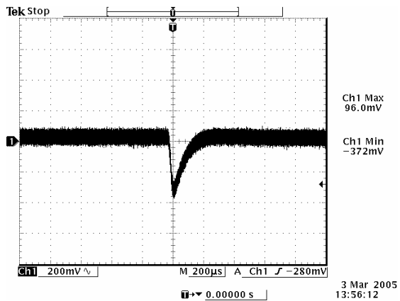
Transients 25% to 50% load 12 Vdc output
