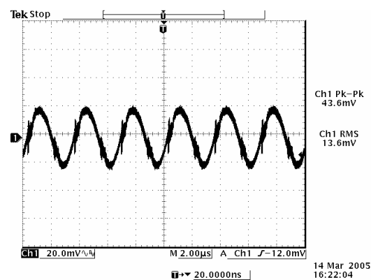
Ripple and noise at max load 2.5 Vdc/25 A output
