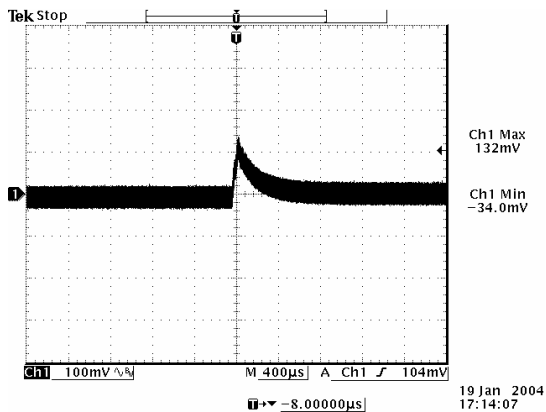
Transients 50% to 25% load 3.3 Vdc output
