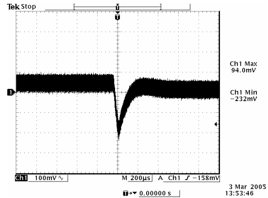
Transients 25% to 50% load 5.0 Vdc output
