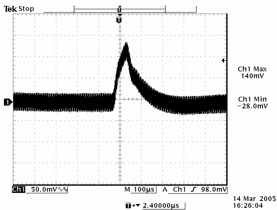
Transients 50% to 25% load 2.5 Vdc output
