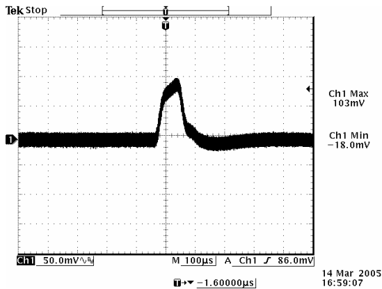
Transients 50% to 25% load 1.5 Vdc output
