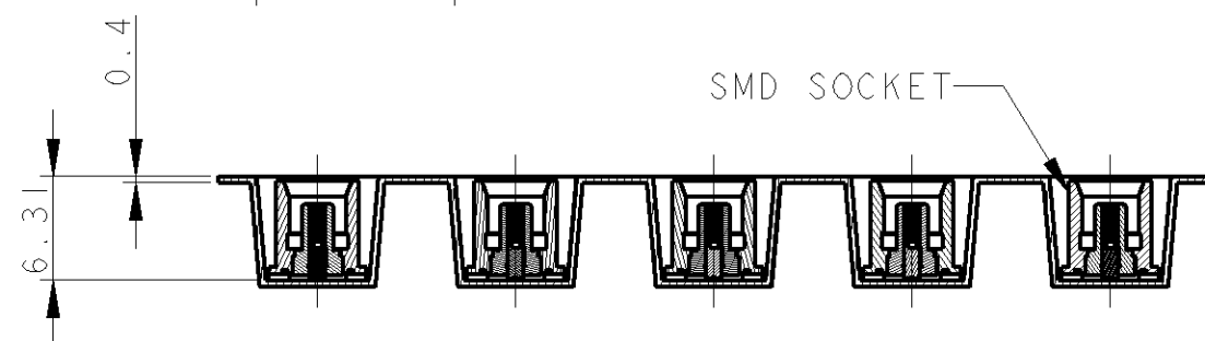
SECTION Y-Y
