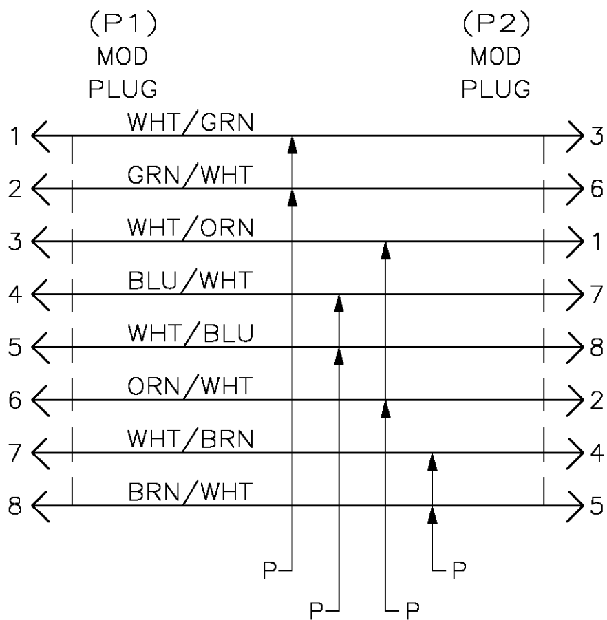
WIRING DIAGRAM CROSSOVER
