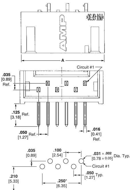
Recommended Mounting Hole Size and Pattern for .062 [1.57] Thick PC Board
