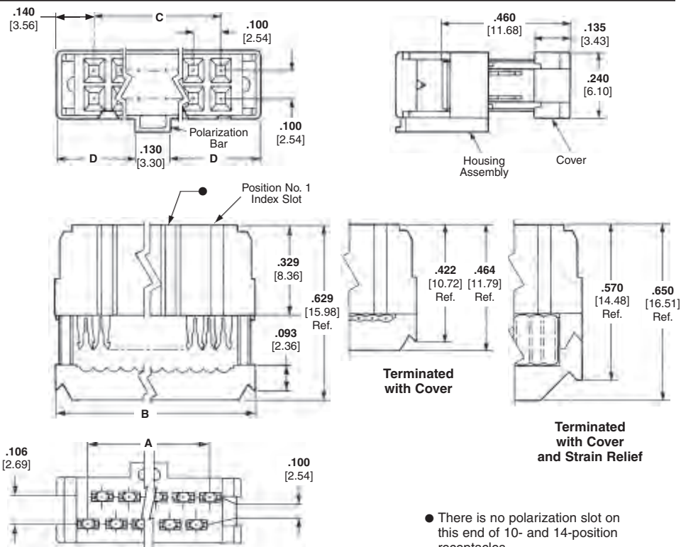
Housing Assembly and Cover
