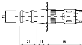
34 push-pull illuminated switch 45 mm page 607
