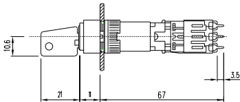
26 keylock switch 2 positions 45 - 70 mm page 598
