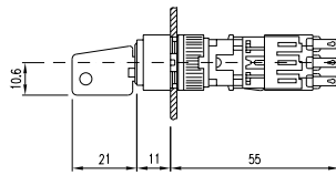
25 keylock switch 2 positions 45 - 70 mm page 598
