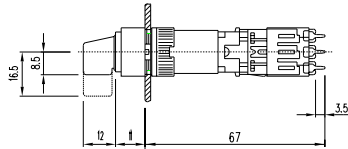
32 selector switch 2 positions 45 - 70 mm page 603
