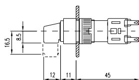
29 selector switch 2 positions 45 - 70 mm page 603
