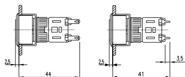
35 indicator actuator 41-44 mm for flush mounting, illuminated-/pushbutton actuator 41-44 mm for flush mounting page 608, 610
