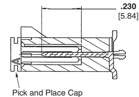
Section K-K
