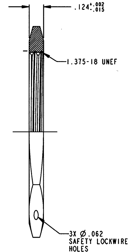
SECTION Z-Z
