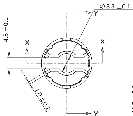
SECTION Y-Y
