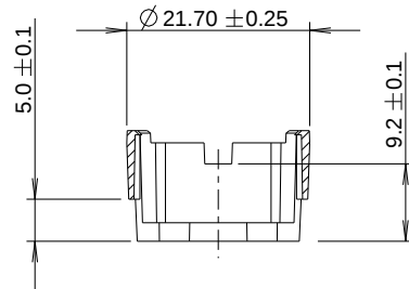
SECTION X-X
