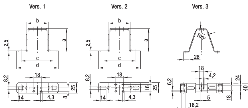
Mounting bracket - foot measure 18 mm (multi-function design)
