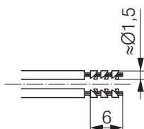
Core crimp sleeve
