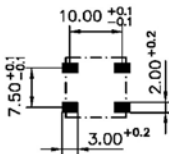
J-lead
