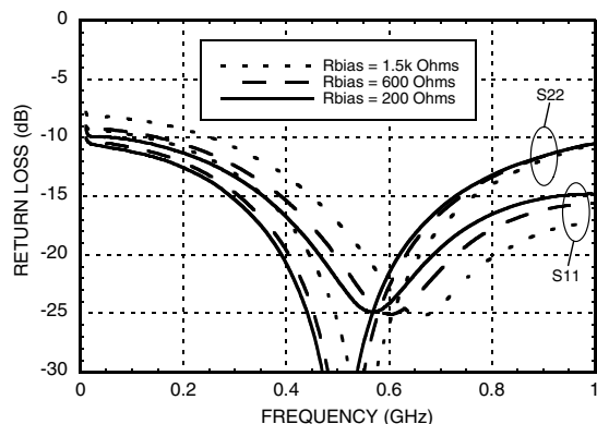
Return Loss vs. R_{bias}
