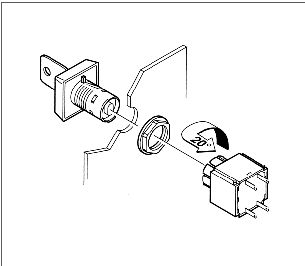
Assembly/Disassembly
