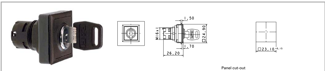
Panel cut-out
