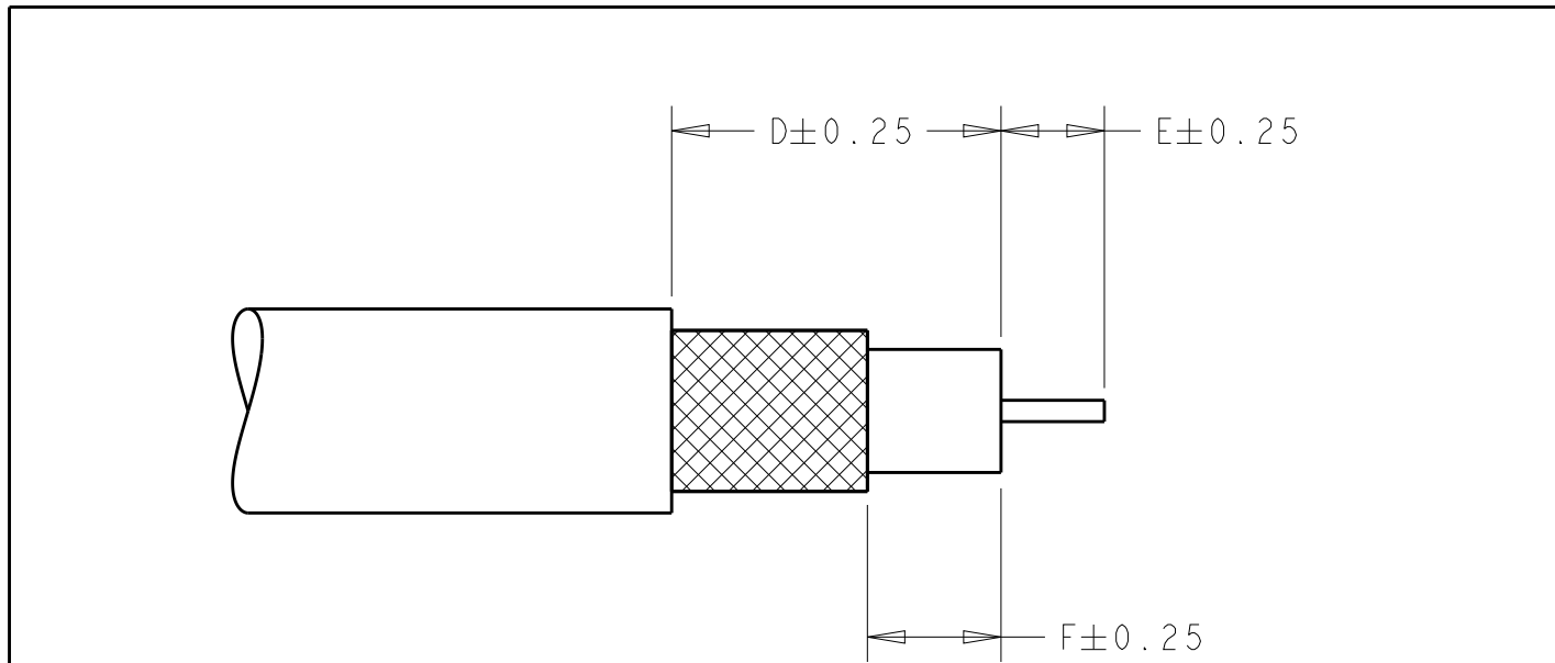
RECOMMENDED STRIP LENGTH DIMENSIONS SCALE: NTS
