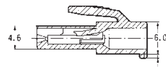
Section X-X
