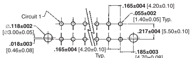
PCB Layout: Component Side (shown with pegs) Recommended Board Thickness .070 [1.78]
