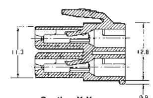
Section X-X
