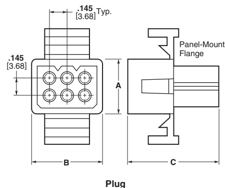
Plug
