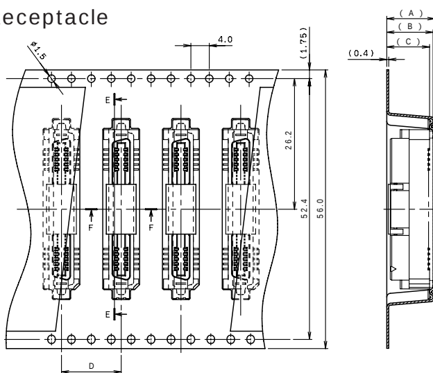
SECT. E-E
