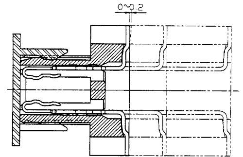
SECT. X-X
