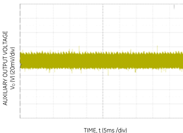
Figure 4. Typical auxiliary 3.3V output ripple and noise ( V_{IN} = 230V_{ac} , 100% load).
