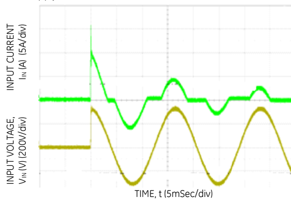
Figure 2. Inrush Current ( V_{IN} = 230V_{ac} , 100% load)
