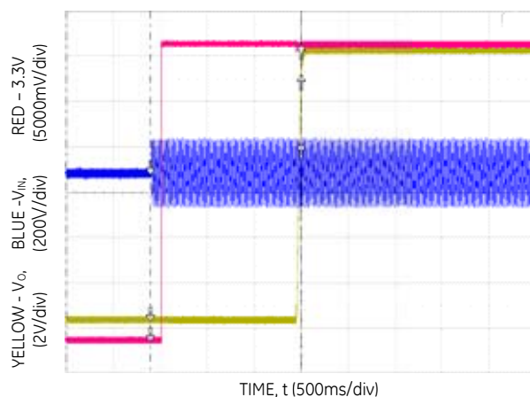
Figure 6. Typical Start-up ( V_{IN} = 150V_{ac} )
