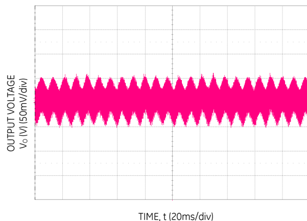
Figure 3. Typical 12V output ripple and noise ( V_{IN} = 230V_{ac} , 100% load).
