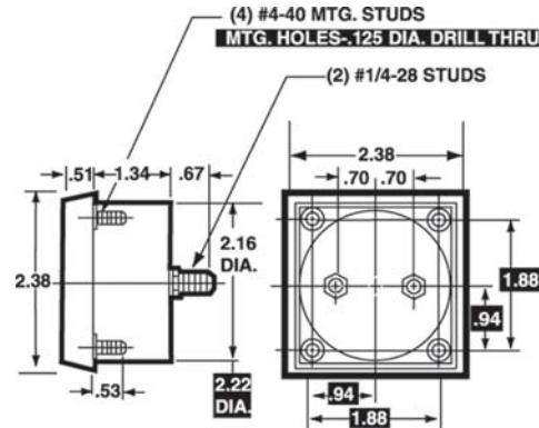
2-1/2"-Models 2122, 2122T, 2142, 2152, 2182
