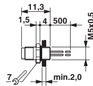
Dimensional drawing
