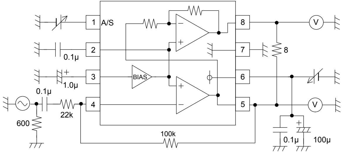
Fig.2 BH7824FVM
