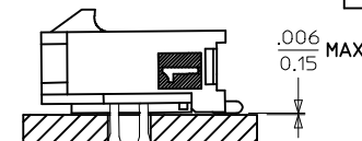
COPLANARITY DETAIL SEE NOTE #7
