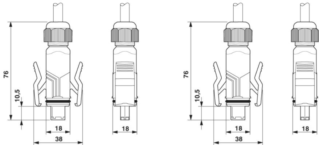
FireWire plug connector, IP67
