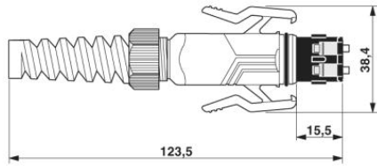
SCRJ plug connector, GOF, IP67
