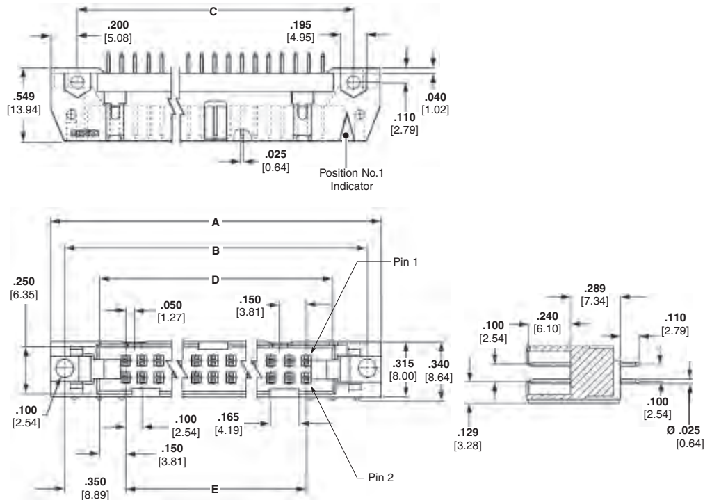
Right-Angle PCB Mount
