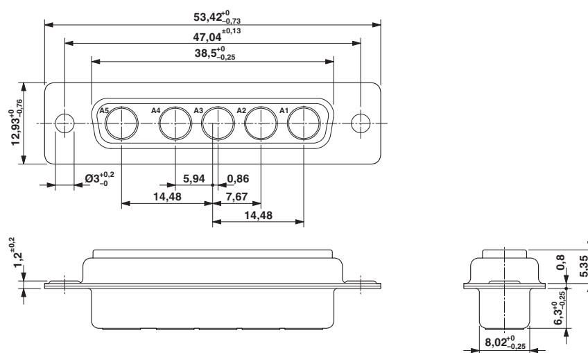
Dimensional drawing
