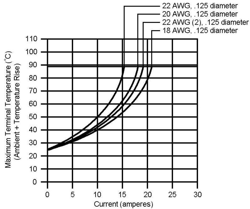
Figure 3 Temperature Rise vs Current Requirements
