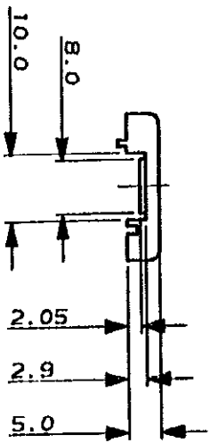
VIEW "A"
