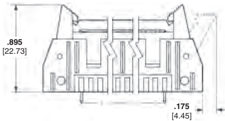
Figure 2 — Use Short Latch for AMP-LATCH Novo Receptacles without Strain Relief & Female Socket Connectors without Strain Relief
