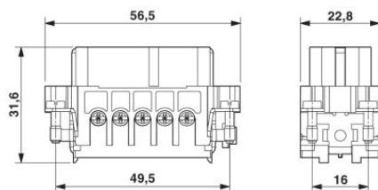
Female insert
