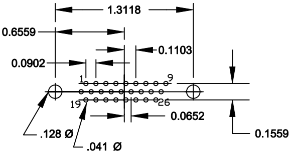
26 POSITION MALE
