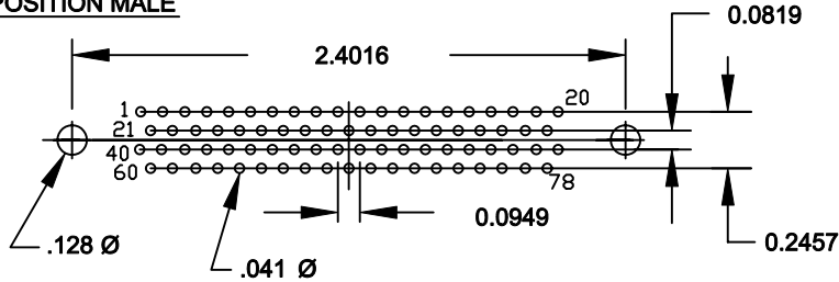
78 POSITION MALE
