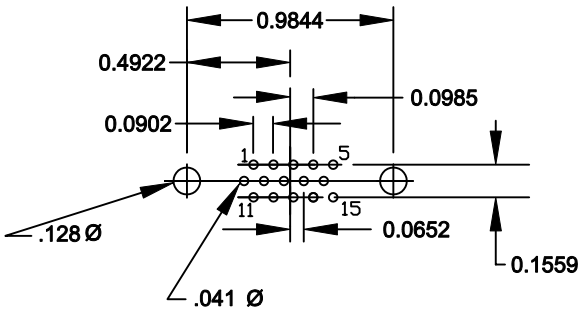
15 POSITION MALE
