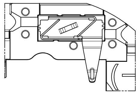
DETAIL 1 SCALE 4:1
