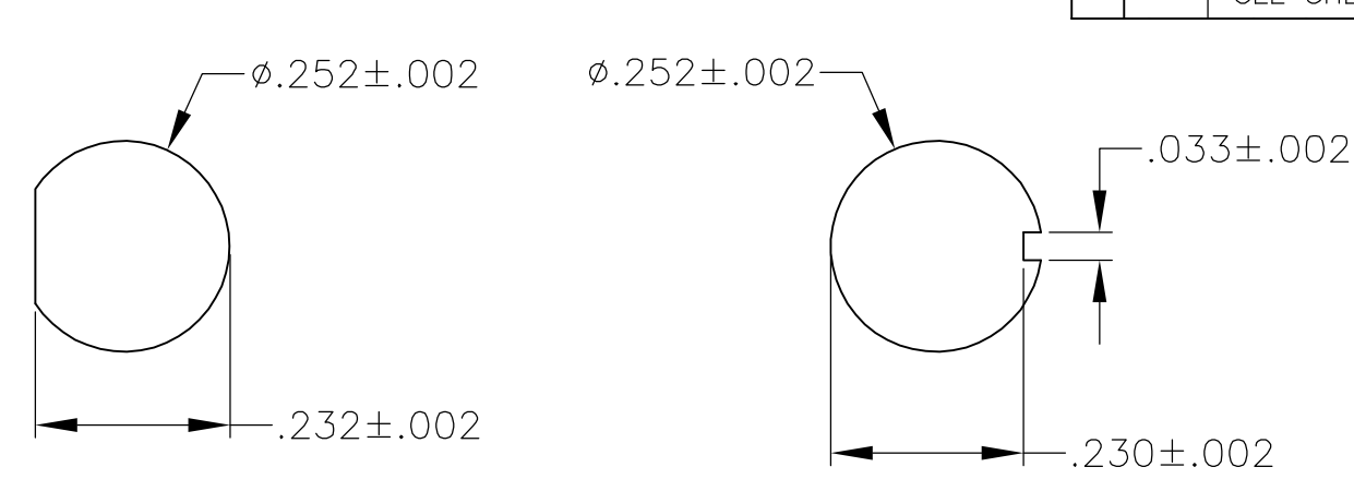
RECOMMENDED PANEL LAYOUTS
