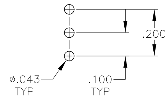
RECOMMENDED PCB LAYOUT TOLERANCES +/- .002
