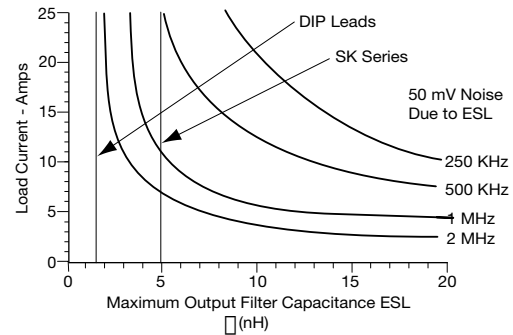
Absolute Maximum Capacitance ESI Assuming no ESR - Capacitive Induced Ripp
