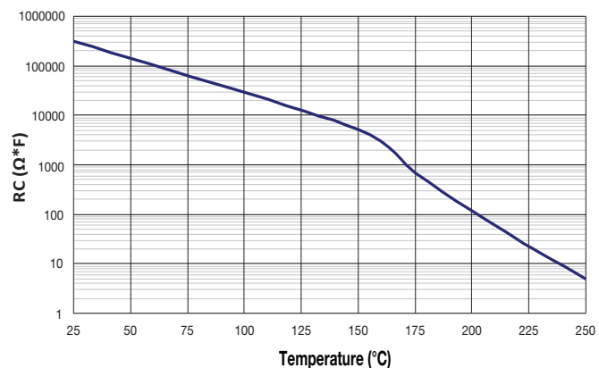
Typical RC vs Temperature (C0G Dielectric)
