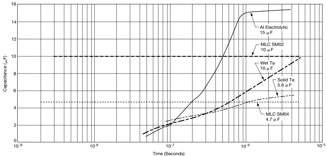
Capacitance as Measured from dv/dt Slope
