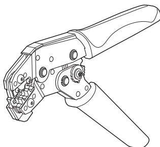
Product drawing
