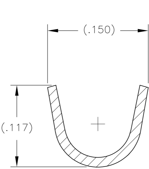
SECTION X-X
