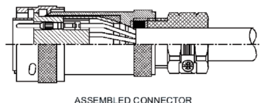
ASSEMBLED CONNECTOR
