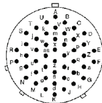
Shell Size 24 48
