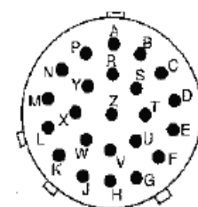
Shell Size 18 23
