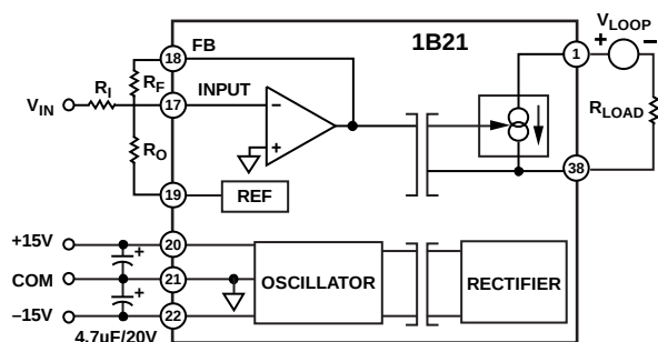
Figure 4. Basic Interconnections
