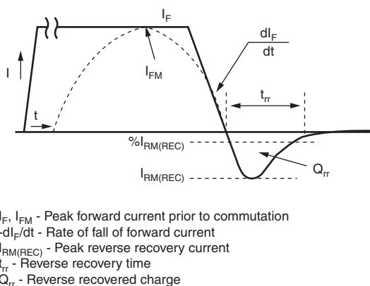
Fig. 4 - Reverse Recovery Time Test Waveform
