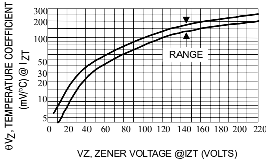
Fig. 2-TEMPERATURE COEFFICIENT-RANGE FOR UNITS 6 TO 51 VOLTS
